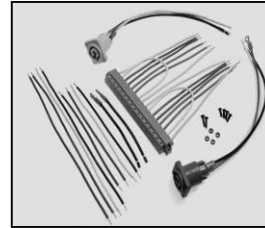
L4.84087AE Cable harness DMX 120 V Kabelbaum DMX 120 V
