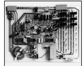
L4.82567.E HF-base drive board HF-Ansteuerung
