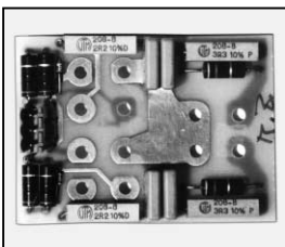
L4.82568.E HF-snubber board HF-Entlastung
