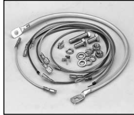
L4.79119.E Connecting wire Verbindungslitzen
