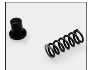
L4.79748.E Door spring + pin Torfeder + Federbolzen
