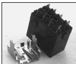
L4.75737.E (BU12AR) Power Relay VC 20 3A Schütz VC 20 3A
