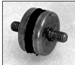
L4.75723.E (BCA 4000+6000+BU12) Shock absorber-set (5 pieces) Schwingmetall-Set (5 Stück)
