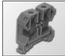
L4.75777.E (BCA 6000) Terminals-set SAK 16/35 (5 pieces) Klemmen-Set SAK 16/35 (5 St.)
