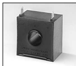
L4.82387.E Current probe (ADM 20) Strommeßspule (ADM 20)
